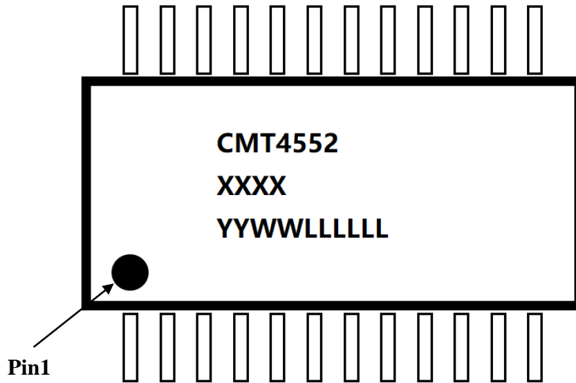
Figure 18: Chip Marking Example
