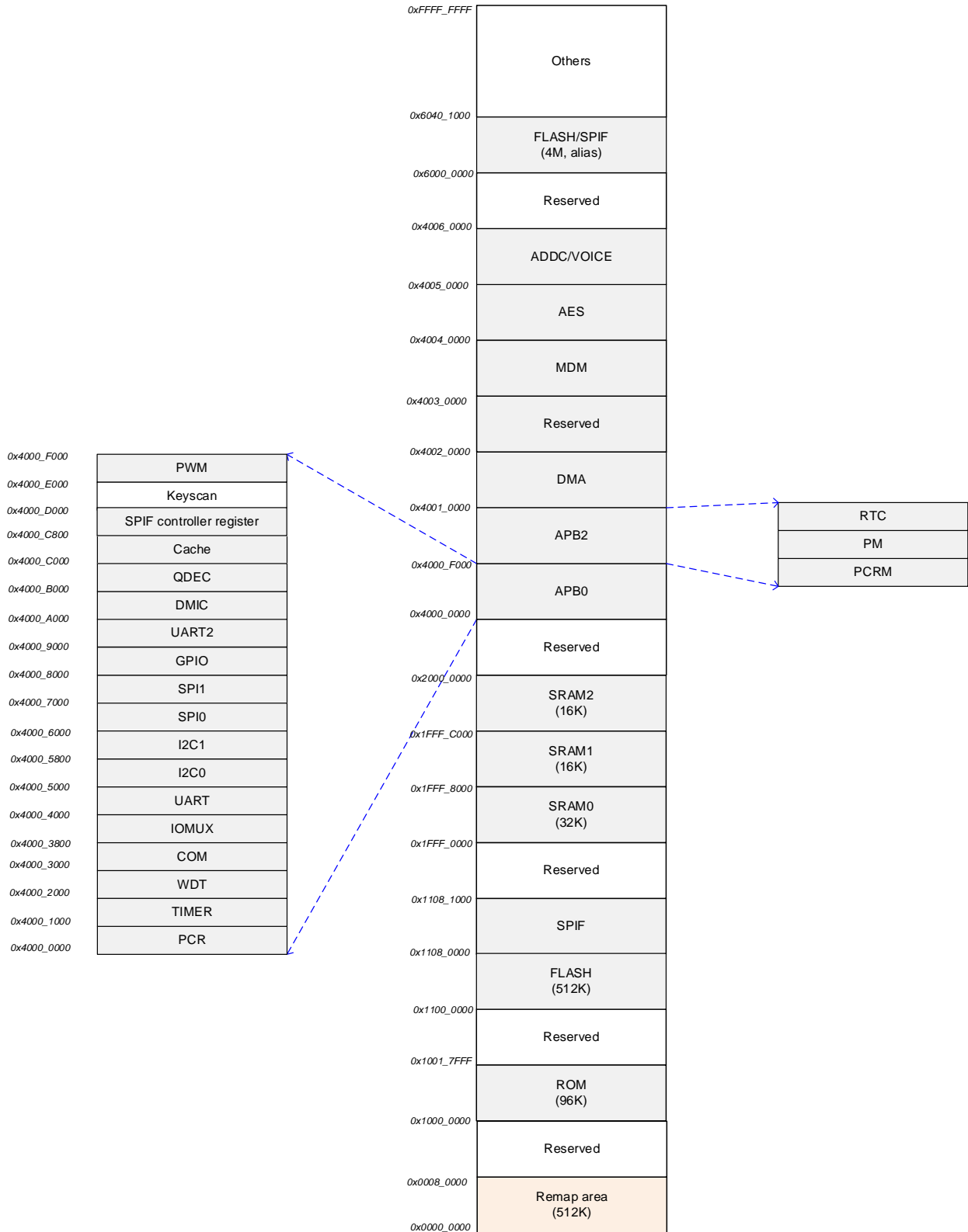
Figure 3: CMT4552 memory space
