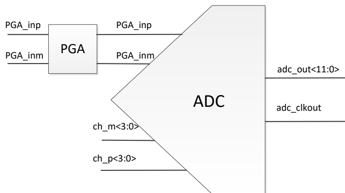
Figure 16: ADC
