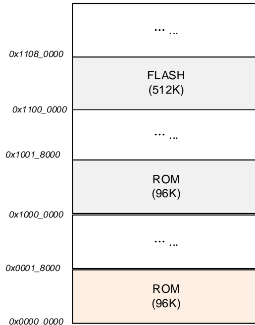
Figure 4: CMT4552 boot mode
