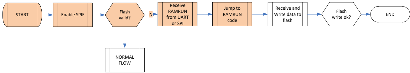
Figure 5: Bootloader flow
