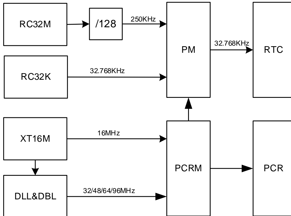
Figure 9: Clock management
