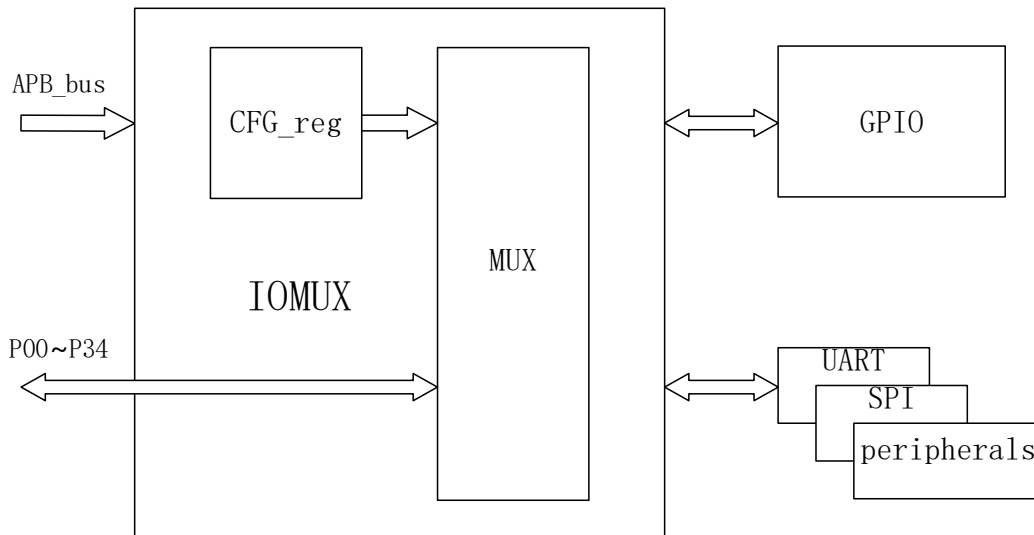
Figure 11: IOMUX structure diagram
