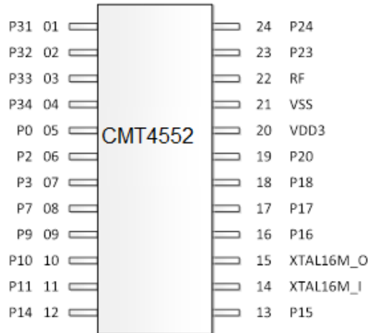
Figure 2: Pin assignment – CMT4552 SSOP24 package
