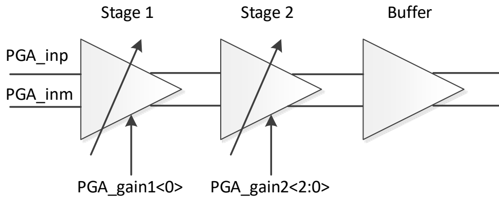
Figure 17: PGA path
